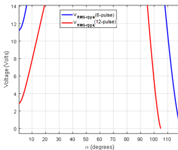
Figure 6. Ripple Voltage for 6-pulses and 12-pulse TRU for compliance with MIL-STD-704F
