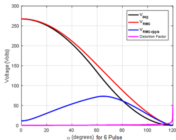
Figure 4. Average Voltage ( V_{avg} ), RMS Voltage ( V_{RMS} ), RMS Ripple Voltage ( V_{RMS\_ripple} ), Distortion Factor ( V_{RMS} / V_{avg} ) for 6-pulse TRU
