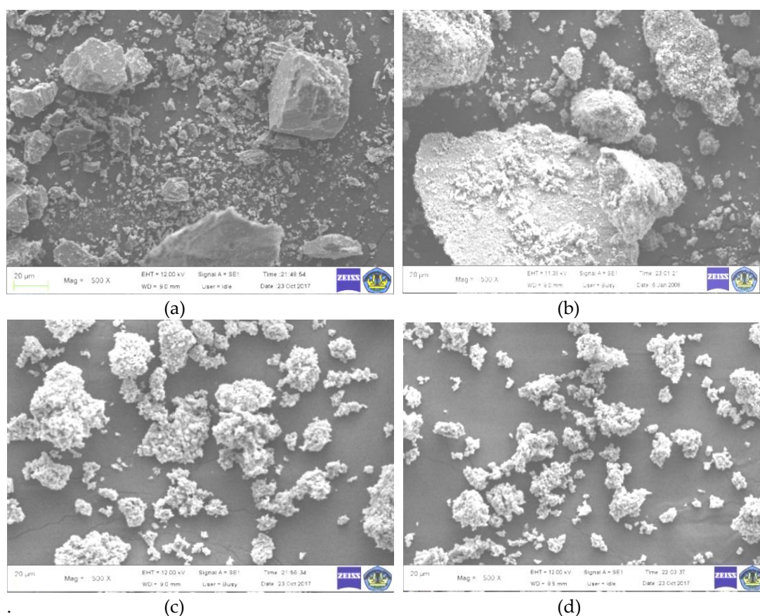
Figure 3. SEM morphology 500x (a) Local limestone powder, (b) Sintering 600°C for 2 hours, (c) Milling speed 300 rpm for 3 hours with sintering temperature 800°C for 3 hours, (d) sintering 1000°C for 4 hours
