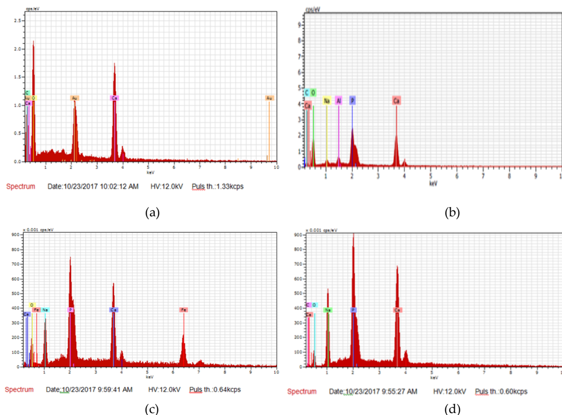
Figure 4. EDX graph on (a) Local limestone, (b) Sintering 600°C for 2 hours, (c). Sintering 800°C for 3 hours, (d) Sintering 1000°C for 4 hours
