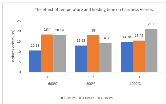
Figure 1. Graph of the effect of sintering and holding time on the hardness of HA (Hydroxyapatite)
