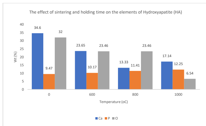
Figure 2. Effect of sintering on the (HA) element of hydroxyapatite
